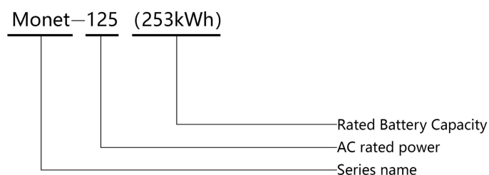
Figure 1-1 Model identification
